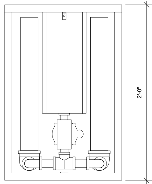
2 BIGSHOTS® DOUBLE BARREL FRONT EL SCALE: 1 1/2" = 1'-0"
