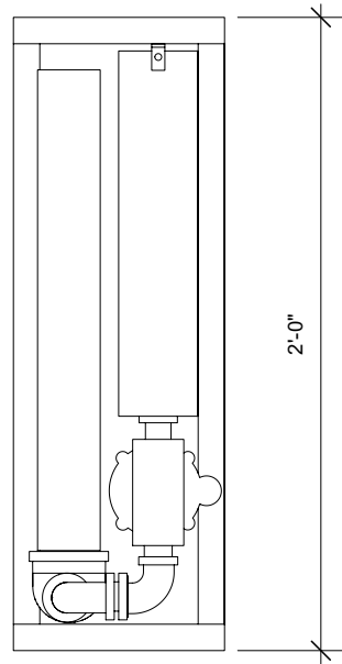
2 BIGSHOTS® SINGLE BARREL FRONT EL SCALE: 1 1/2" = 1'-0"
