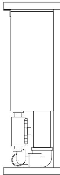
3 BIGSHOTS® SINGLE BARREL SIDE EL SCALE: 1 1/2" = 1'-0"
